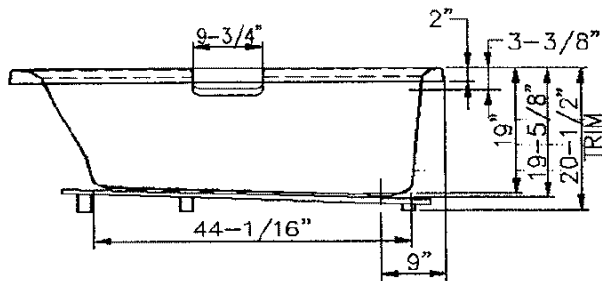
ELEVATION AND PART SECTION
